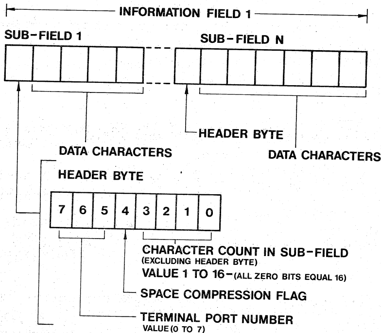
Figure D-3 Terminal Port Encoding Format
