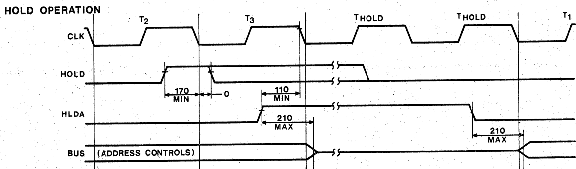
Figure 4-5 8085 Bus Timing
