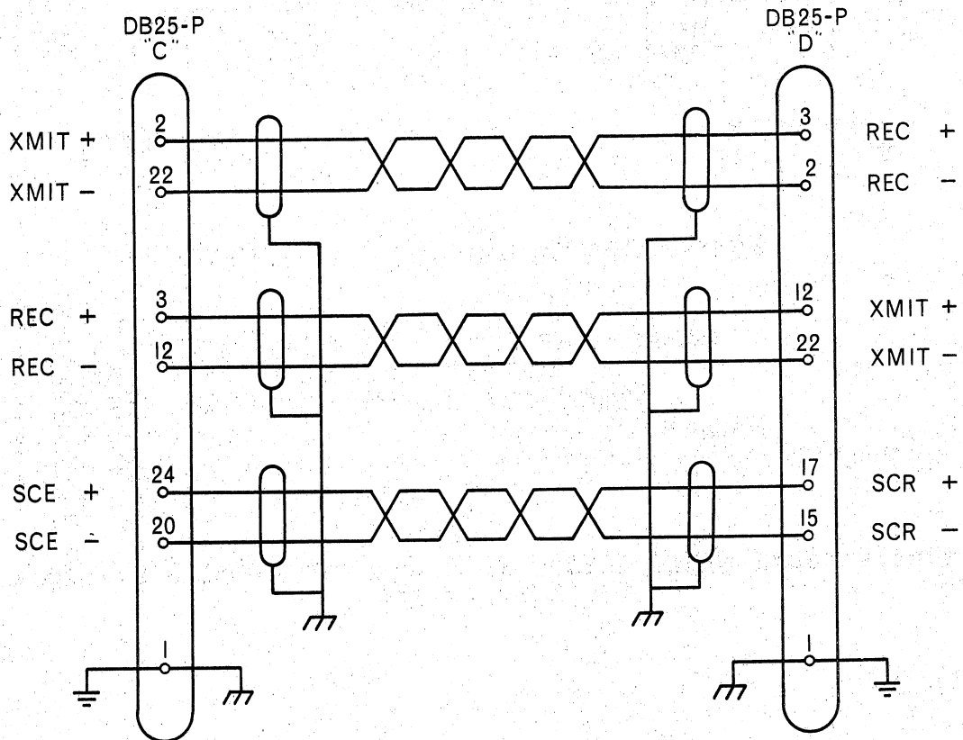
ROUTE-THROUGH RS422 CABLE INTERCONNECTIONS
